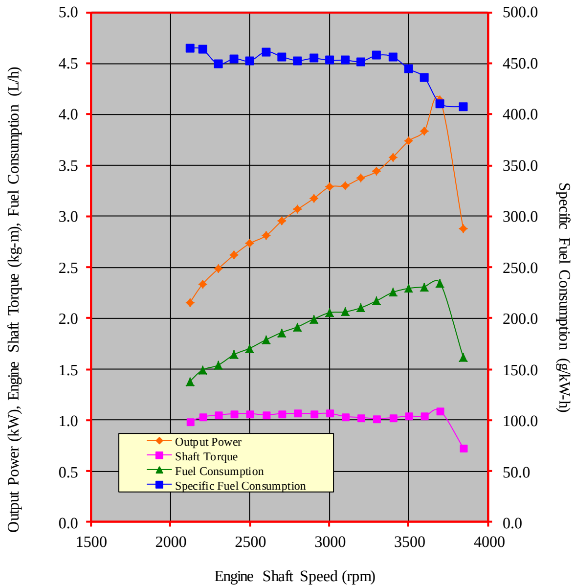
Figure 3. Performance characteristic curves of the YAMADA GT200 gasoline engine
