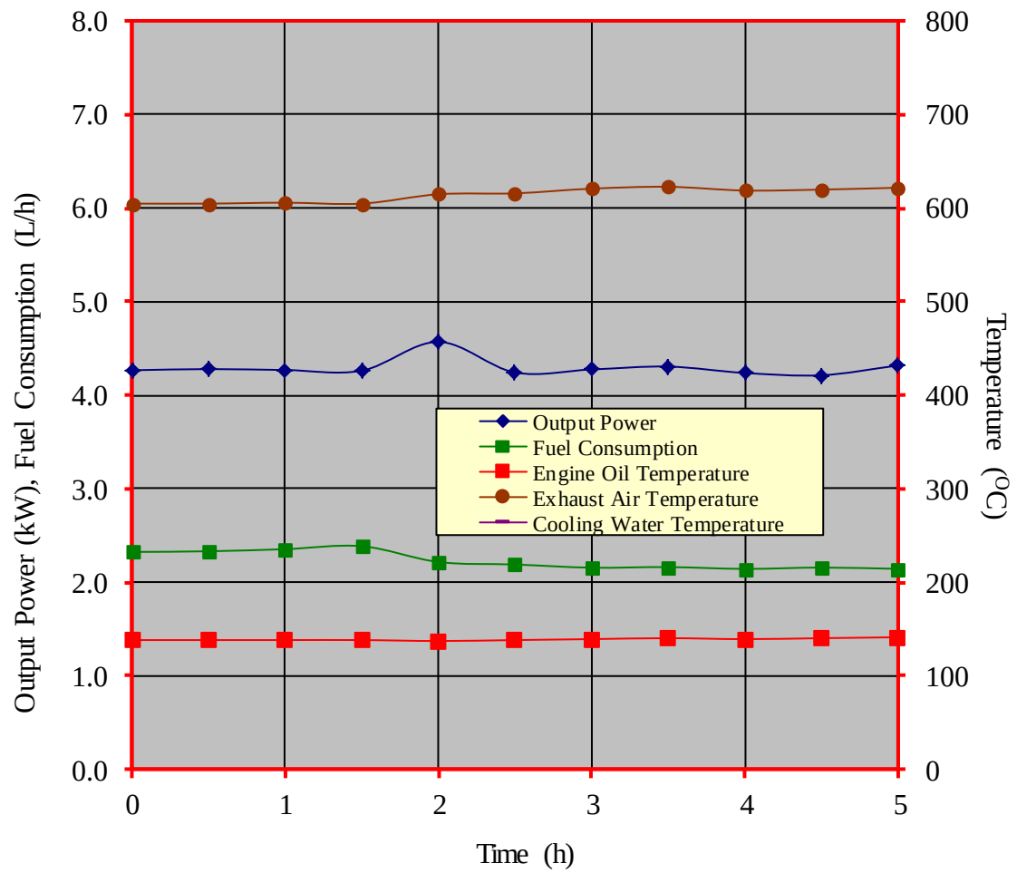
Figure 4. Performance characteristic curves during the continuous running test of the YAMADA GT200 gasoline engine
