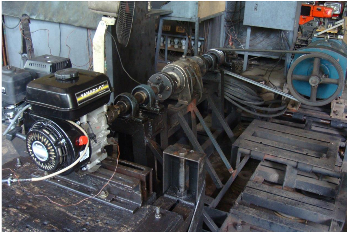
Figure 2. Test set-up of the YAMADA GT200 Gasoline Engine
